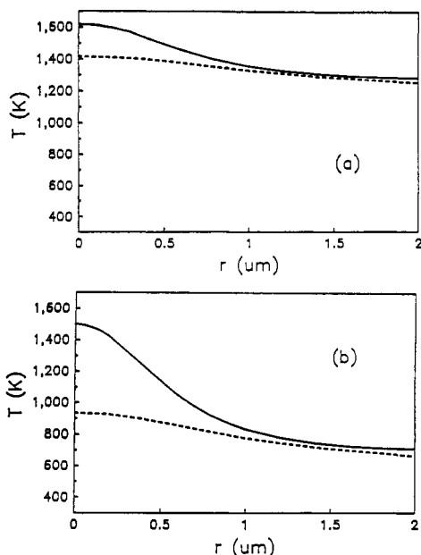
Figure 7. Calculated temperature profiles vs radial displacement ( \mu\text{m} ) for 4- \mu\text{m} -diameter, 0.62- \mu\text{m} -thick polysilicon disks for the top of the disk (solid line) and bottom of the disk (dashed line) for CW laser heating of (a) a fused-silica substrate (488 nm, 24 mW) and (b) a sapphire substrate (514.5 nm, 100 mW). (From ref 25.)
