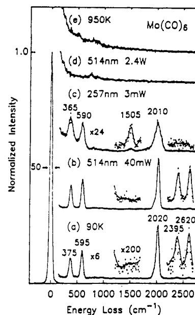
Figure 5. EELS (electron energy loss spectroscopy) spectra of 1.5 L of Mo(CO) 6 on Si(111) 7 \times 7 (a) at 90 K, (b) after 514.5-nm laser irradiation of 40 mW/cm 2 for 20 min, (c) after 257-nm laser irradiation of 3.8 mW/cm 2 for 20 min, (d) after 514.5-nm laser irradiation of 2.4 W/cm 2 for 5 min, and (e) after resistive heating to 950 K. (Reprinted from ref 120; copyright 1988 Gordon & Breach Science Publishers Ltd.)
